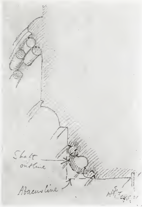
Fig. 207. Arch Moulding of Windows Round Rotunda, Templar's Church, Laon.
